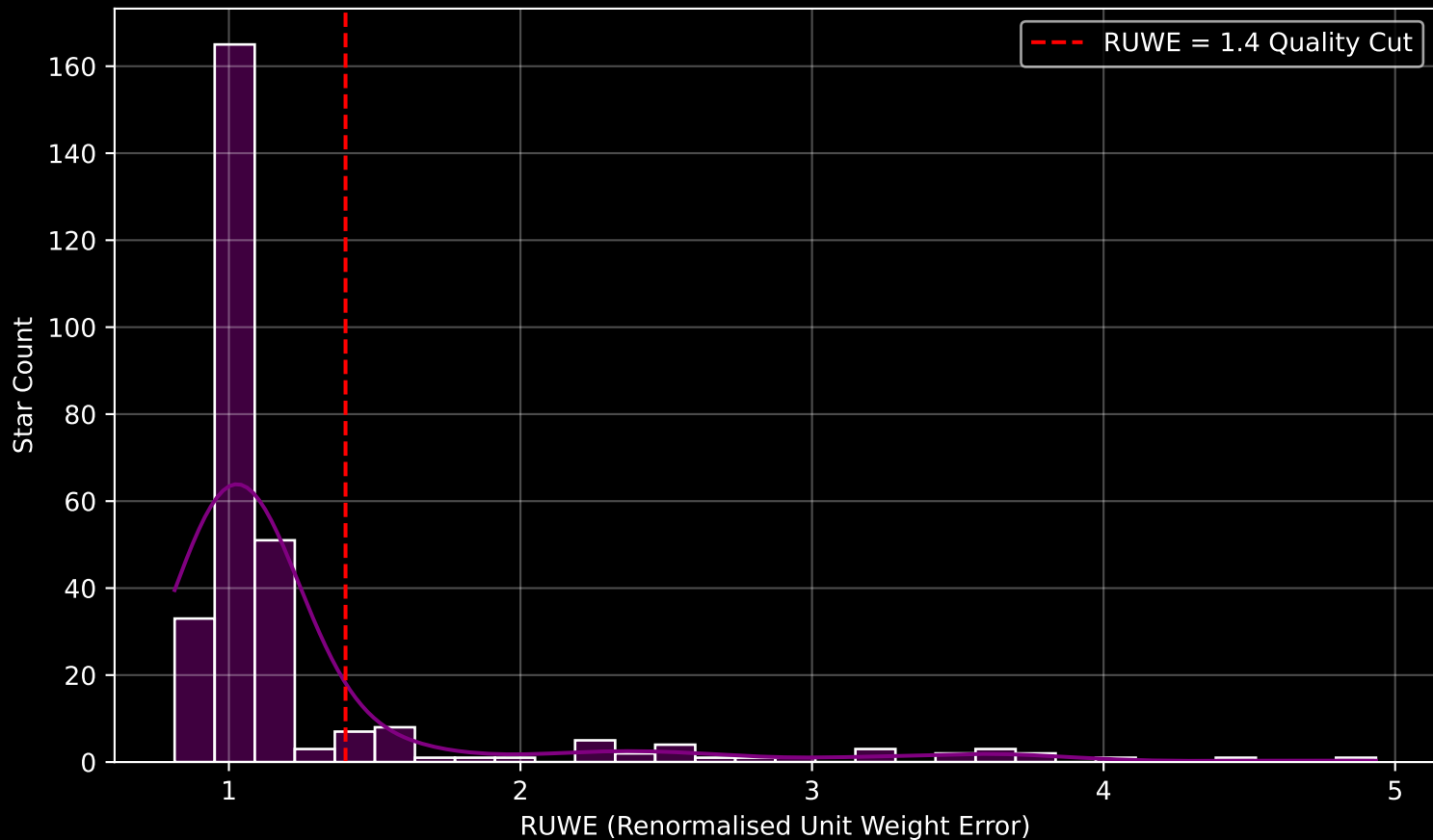
GALAH DR4 Field [7007] RUWE Distribution (n= 297)
