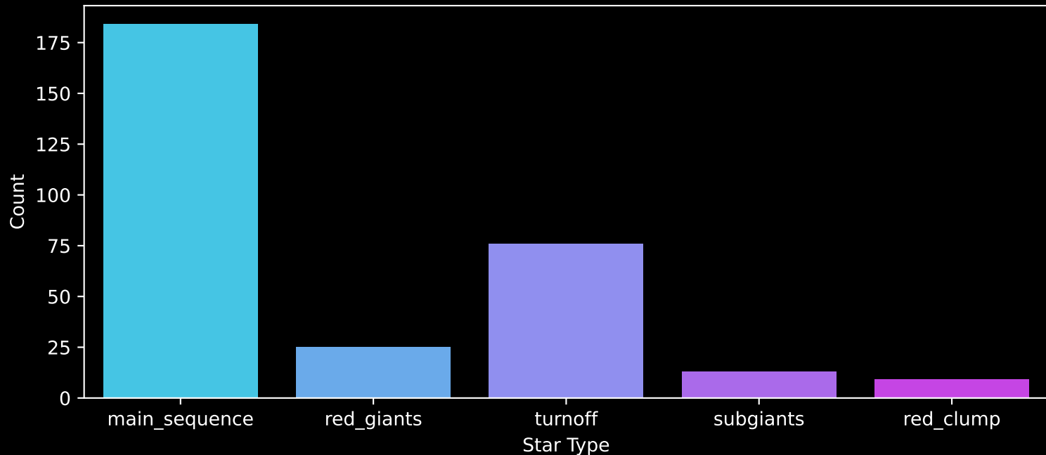
GALAH DR4 Field: [7007] Count plot of Star Type
