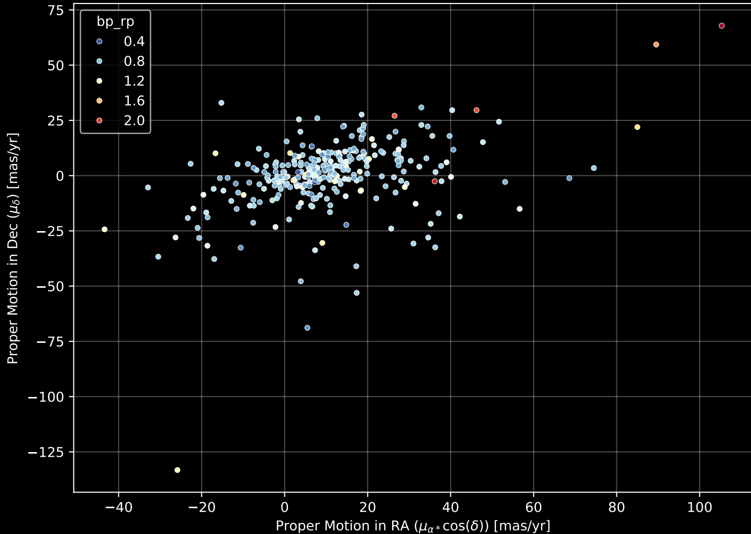
GALAH DR4 Field: [7007] Proper Motion Diagram (n= 307)
